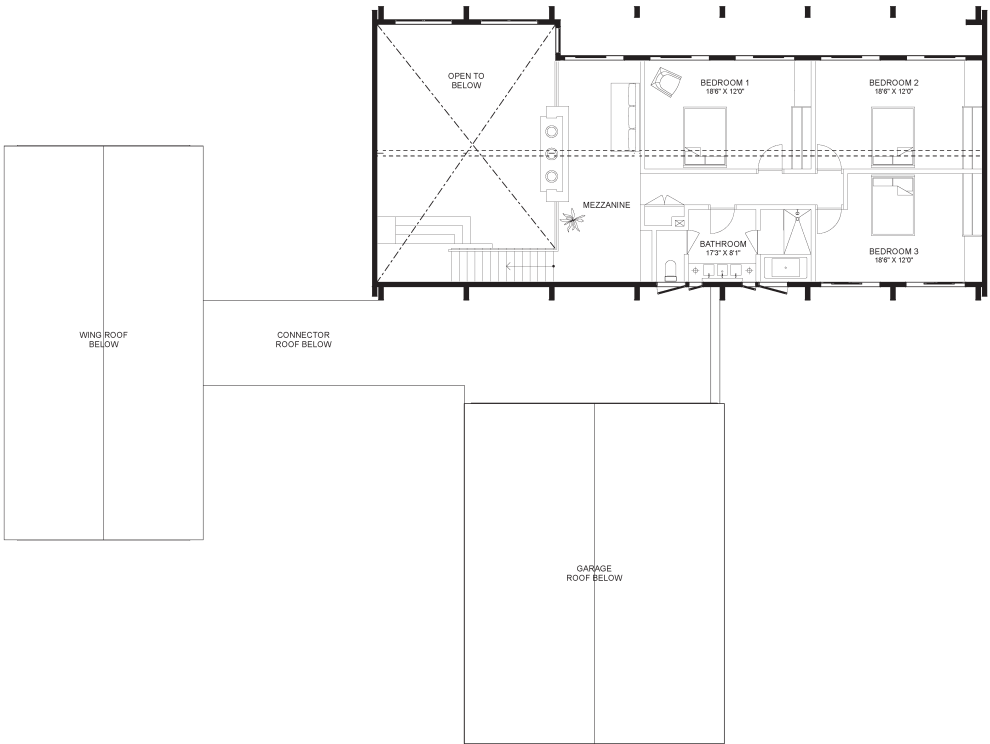
SECOND FLOOR
