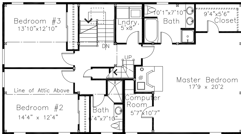
Second Floor
