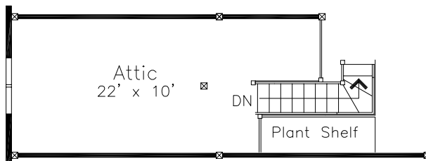
Attic Floor
