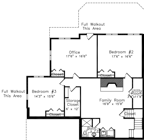
Basement Floor
