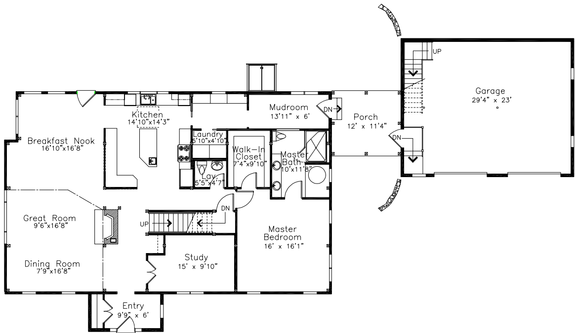
First Floor
