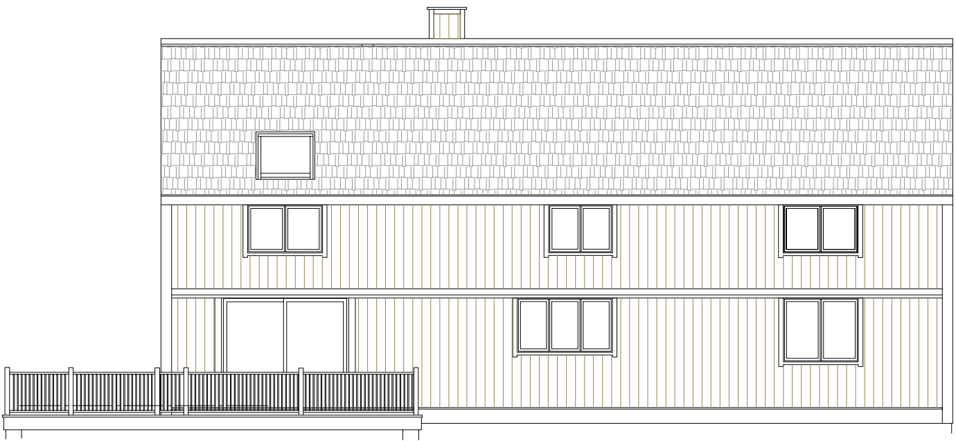
Kitchen Side Elevation
