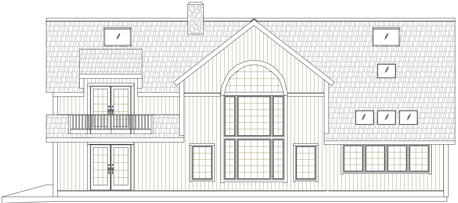
Great Room Side Elevation
