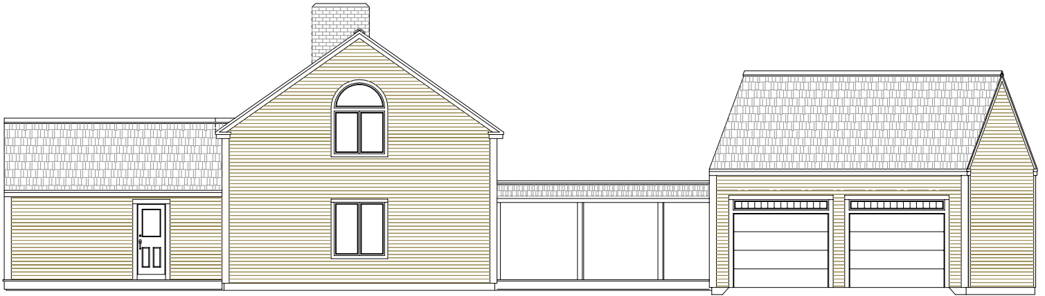
Bedroom End Elevation
