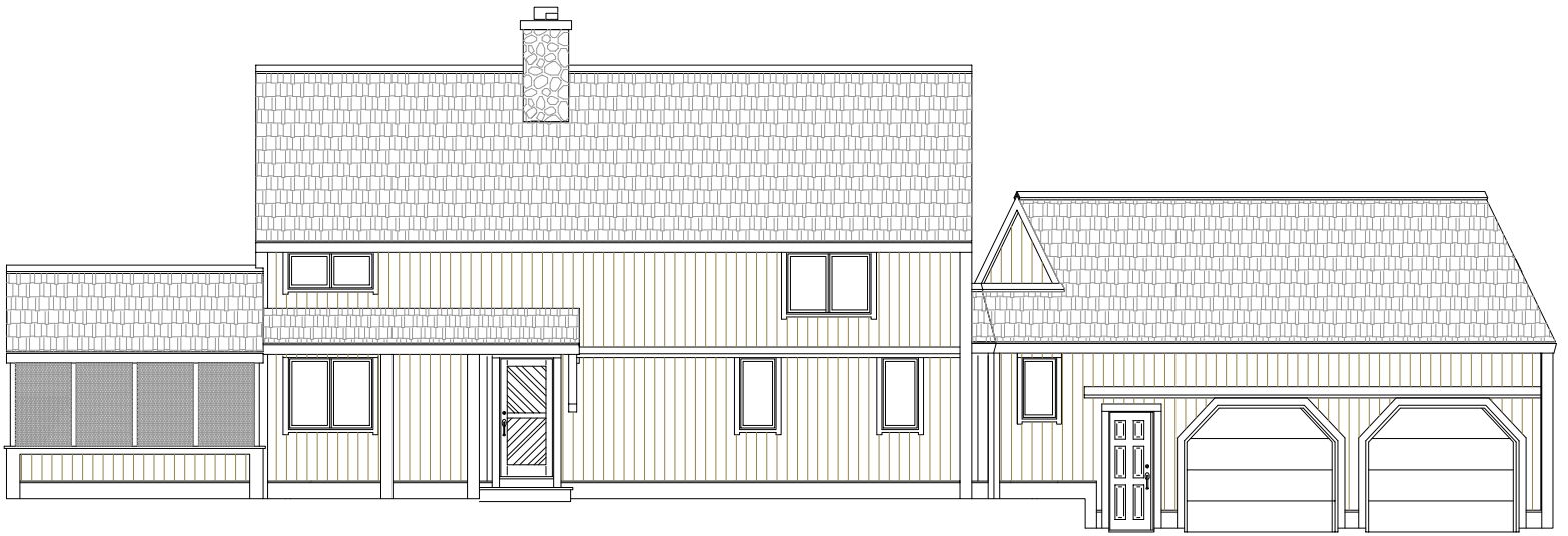
Entry Side Elevation
