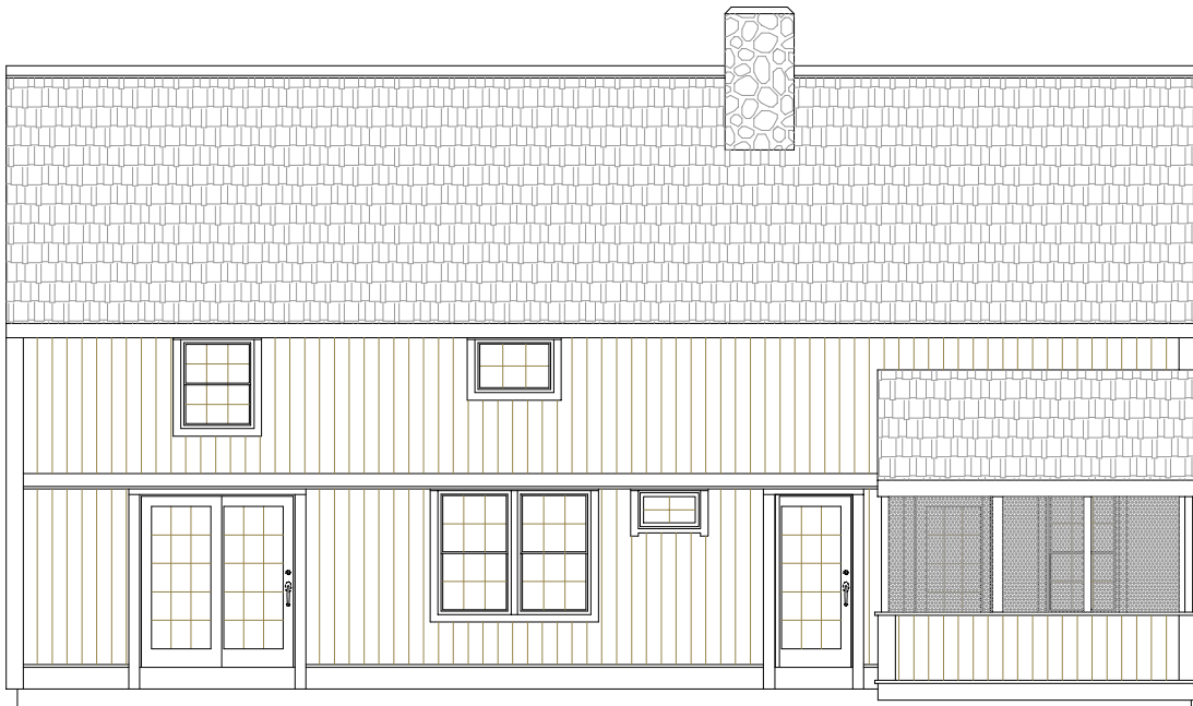
Entry Side Elevation
