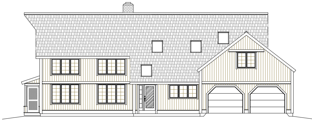
Entry Side Elevation
