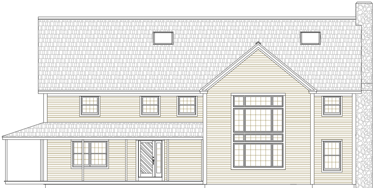
Entry Side Elevation
