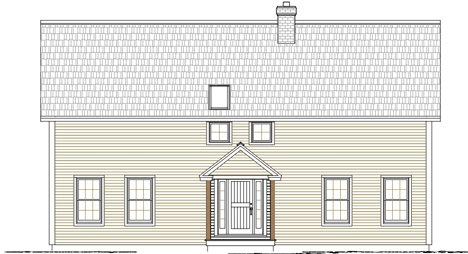
Entry Side Elevation
