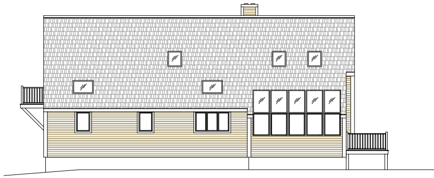
Kitchen Side Elevation
