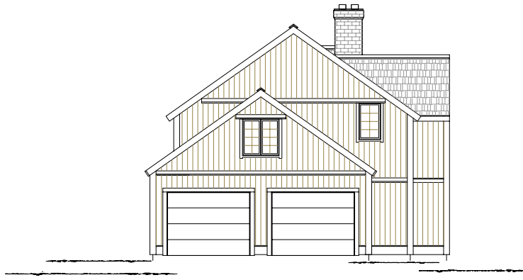
Garage End Elevation www.yankeebarnhomes.com 1-800-258-9786
