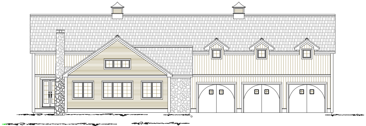
Great Room Side Elevation
