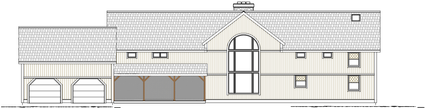
Great Room Side Elevation
