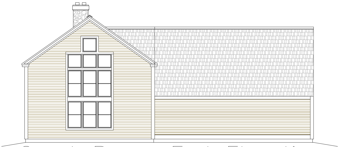
Great Room End Elevation
