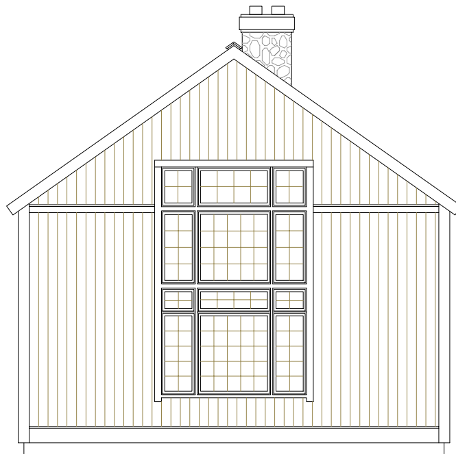
Great Room End Elevation
